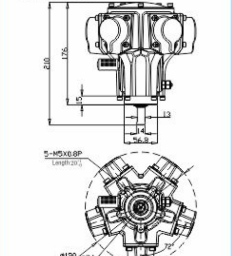
M40/M50 Dimension Diagram Of Air Motor
