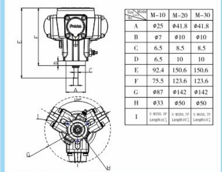
Dimension Diagram Of Air Motor
